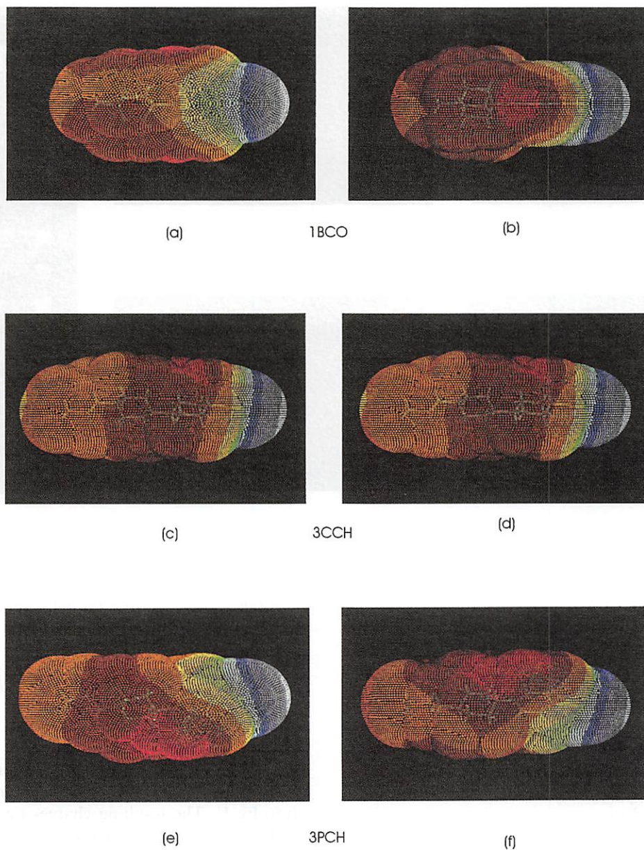
Figure 2. ESP surfaces for 1BCO, (a) and (b); 3CCH (c) and (d); 3PCH (e) and (f); 3CB (g) and (h); and 3OCB (i) and (j). The calculations were performed using the MP2/6-31G**//HF/6-31G* method. The surfaces shown are 2.0 Å above the van der Waals surfaces of the molecules. Each molecule is shown in two perspectives, rotated by 90°, (a–f), or 180°, (g–j) (see figure 2 continued), about the long axis. In (k) the colour coding for the electrostatic potential surfaces is shown. Each colour belongs to a different interval of potential energy of a test charge of 1 |e|.
